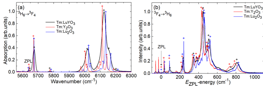
Fig. 9. Low-temperature (LT, 12 K) spectroscopy of Tm^{3+} ions in the LuYO_3 , Y_2O_3 , Lu_2O_3 ceramics: (a) absorption spectra, the {}^3H_6 \rightarrow {}^3F_4 transition; (b) luminescence spectra, the {}^3F_4 \rightarrow {}^3H_6 transition, ZPL – zero-phonon-lines, “+” indicate the assigned electronic transitions.
